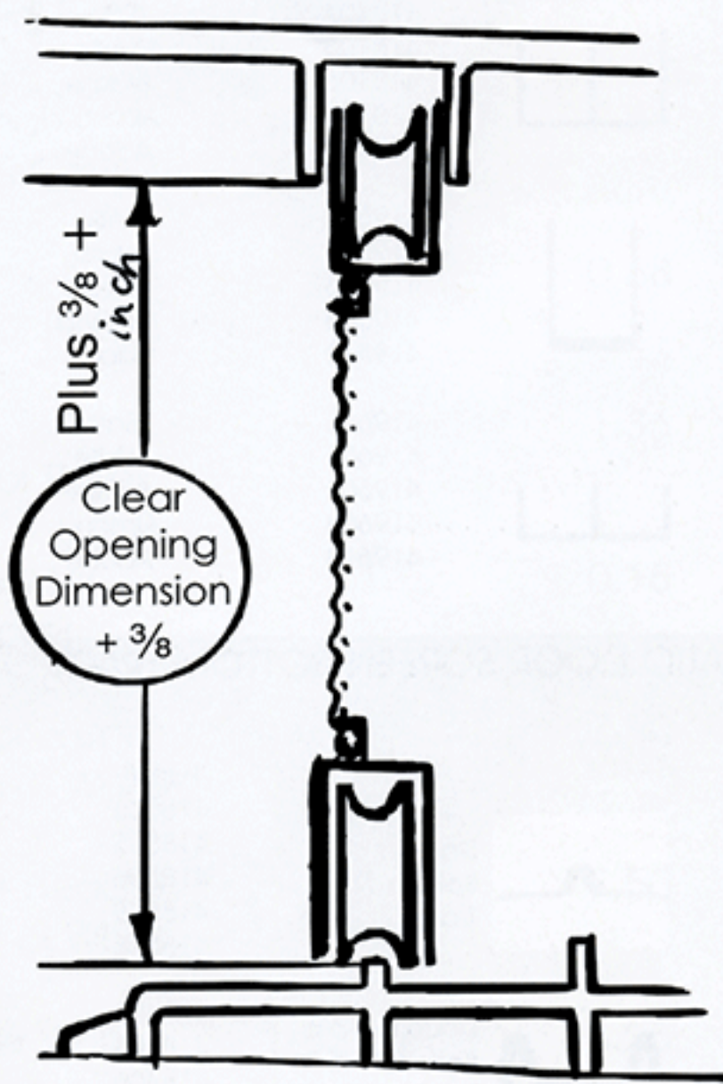
Sill (Bottom)
