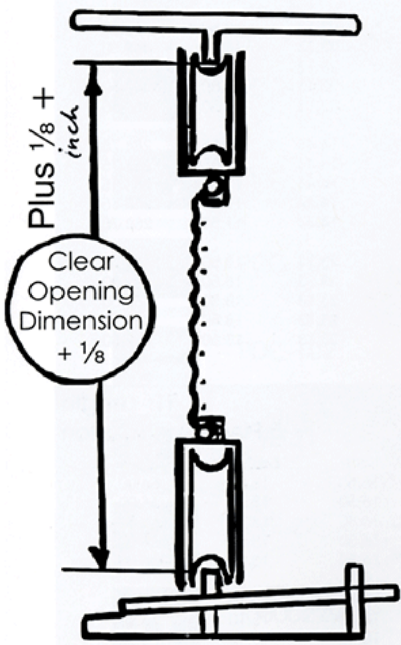
Sill (Bottom)
